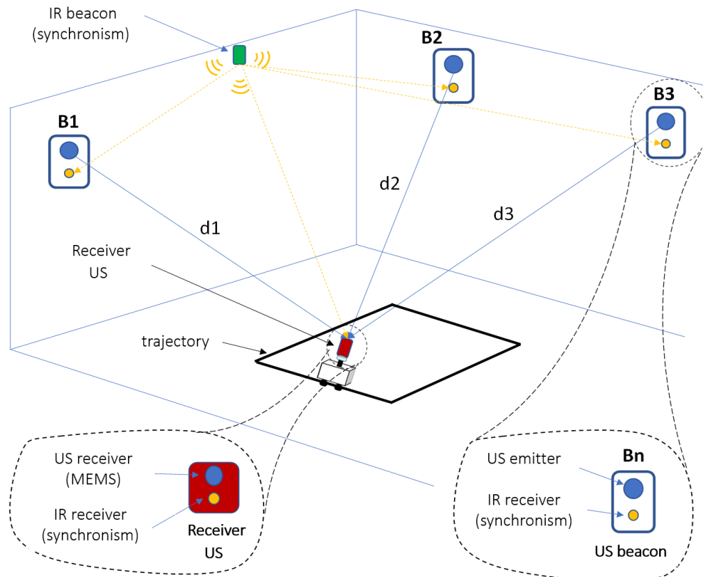
Figure 6.20: Proposed ULPS.
