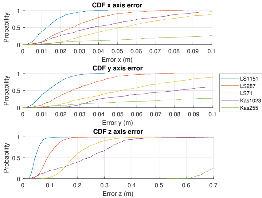
Figure 3.10: CDF for the absolute error in the estimation of the receiver's position in coordinates x , y and z for different types of sequences.
