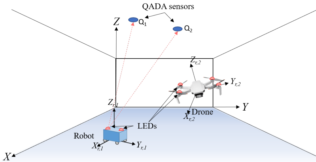
Figure 5.1: General diagram of the proposed positioning system.
