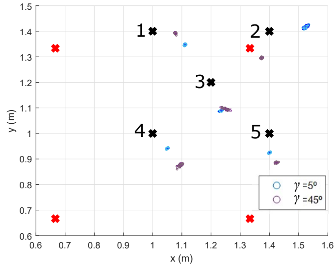
Figure 6.10: Experimental position estimates for \gamma = \{5^\circ, 45^\circ\} with the transmission of a 1151-bit LS sequence with a displacement of 10 samples. The black crosses are the ground-truth, the red crosses represent the projection of the LED beacons and the ellipses at each point are error ellipses with a 95% confidence level.
