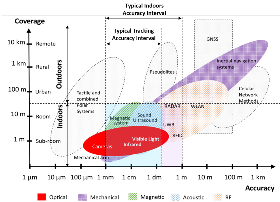
Figure 2.1: Overview of indoor LPS according to accuracy and range (adapted from [Mau12, Lop14, Ure18]).
