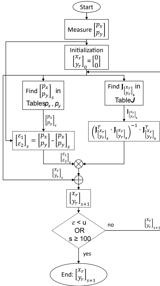
Figure 4.9: Flowchart of the proposed NLSE algorithm.
