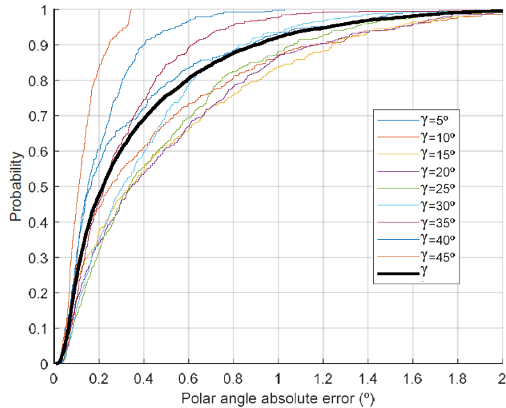
Figure 4.18: Absolute error in the estimation of the polar angle with a SNR of 10 dB for values \gamma = \{5^\circ, 10^\circ, 15^\circ, 20^\circ, 25^\circ, 30^\circ, 35^\circ, 40^\circ, 45^\circ\} at z = 0 m.
